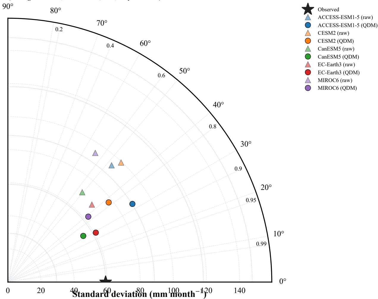
Taylor diagram — monthly climatology, independent validation (triangles = raw, circles = QDM; Taylor 2001)
